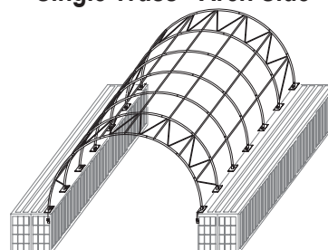
Container Shelter Single Truss - Arch Side
