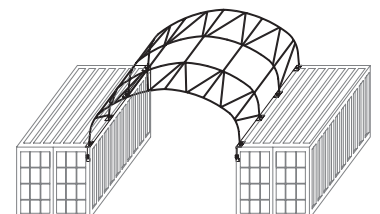
Container Shelter Single Truss - Vertical Side
